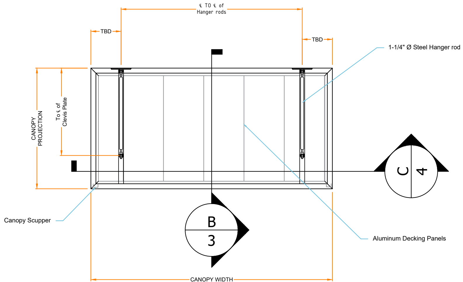
CANOPY PLAN VIEW
