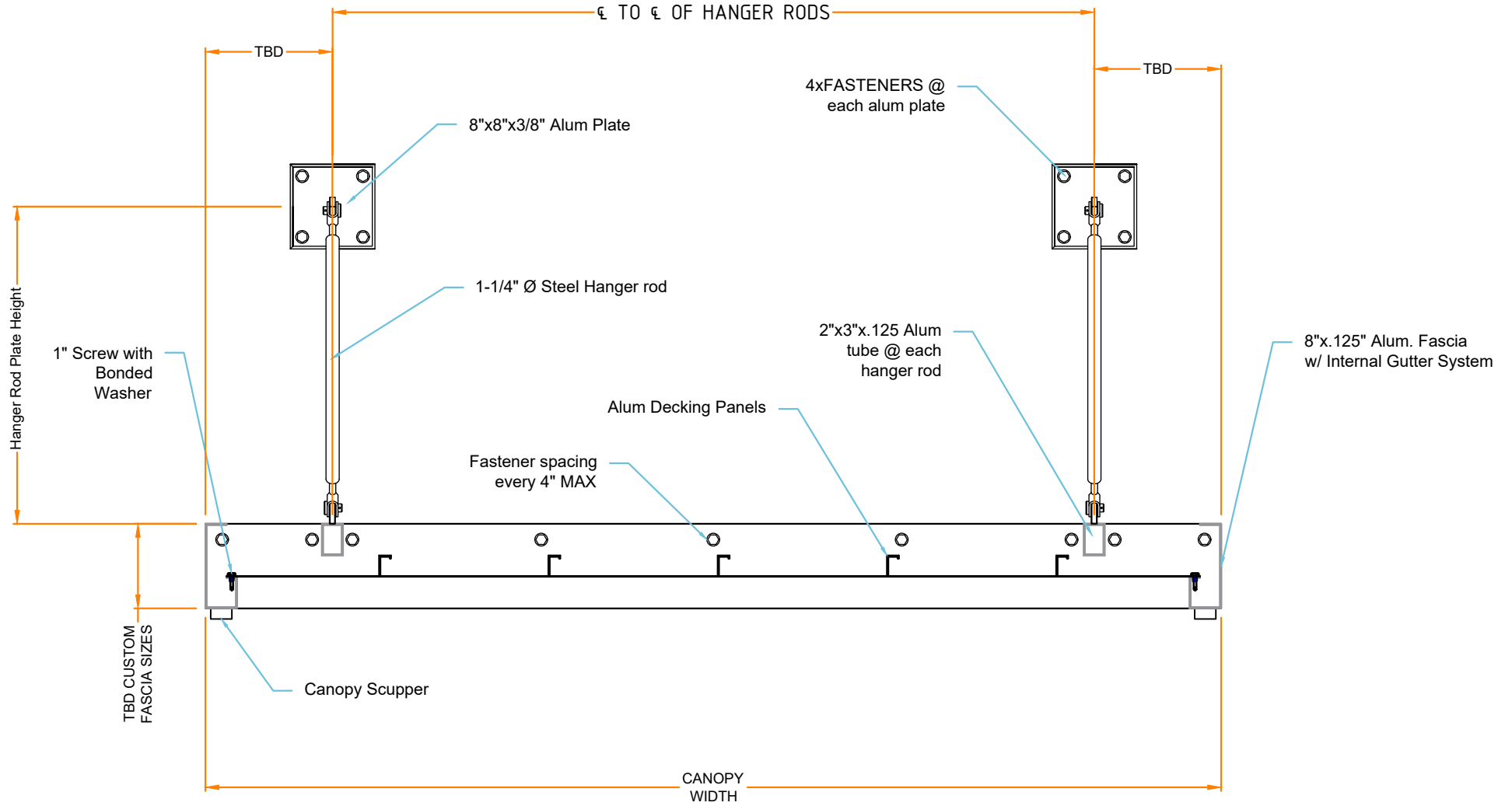
CANOPY FRONT VIEW
