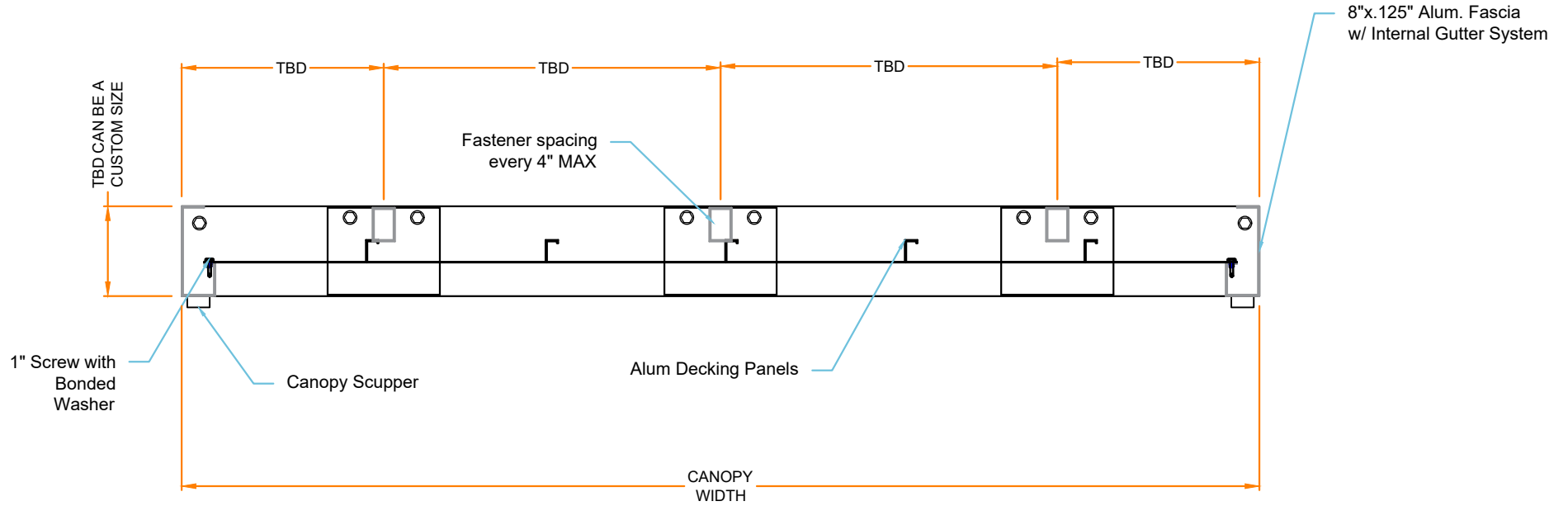
CANOPY FRONT VIEW
