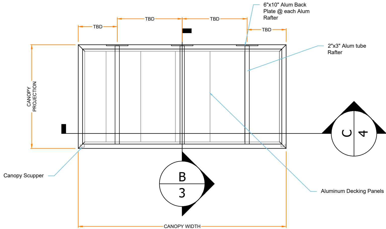
CANOPY PLAN VIEW
