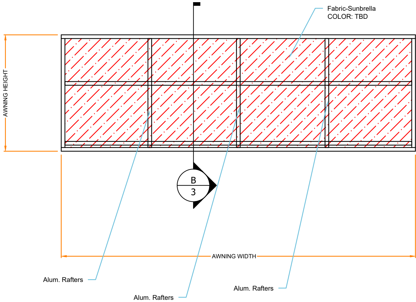
AWNING FRONT VIEW
