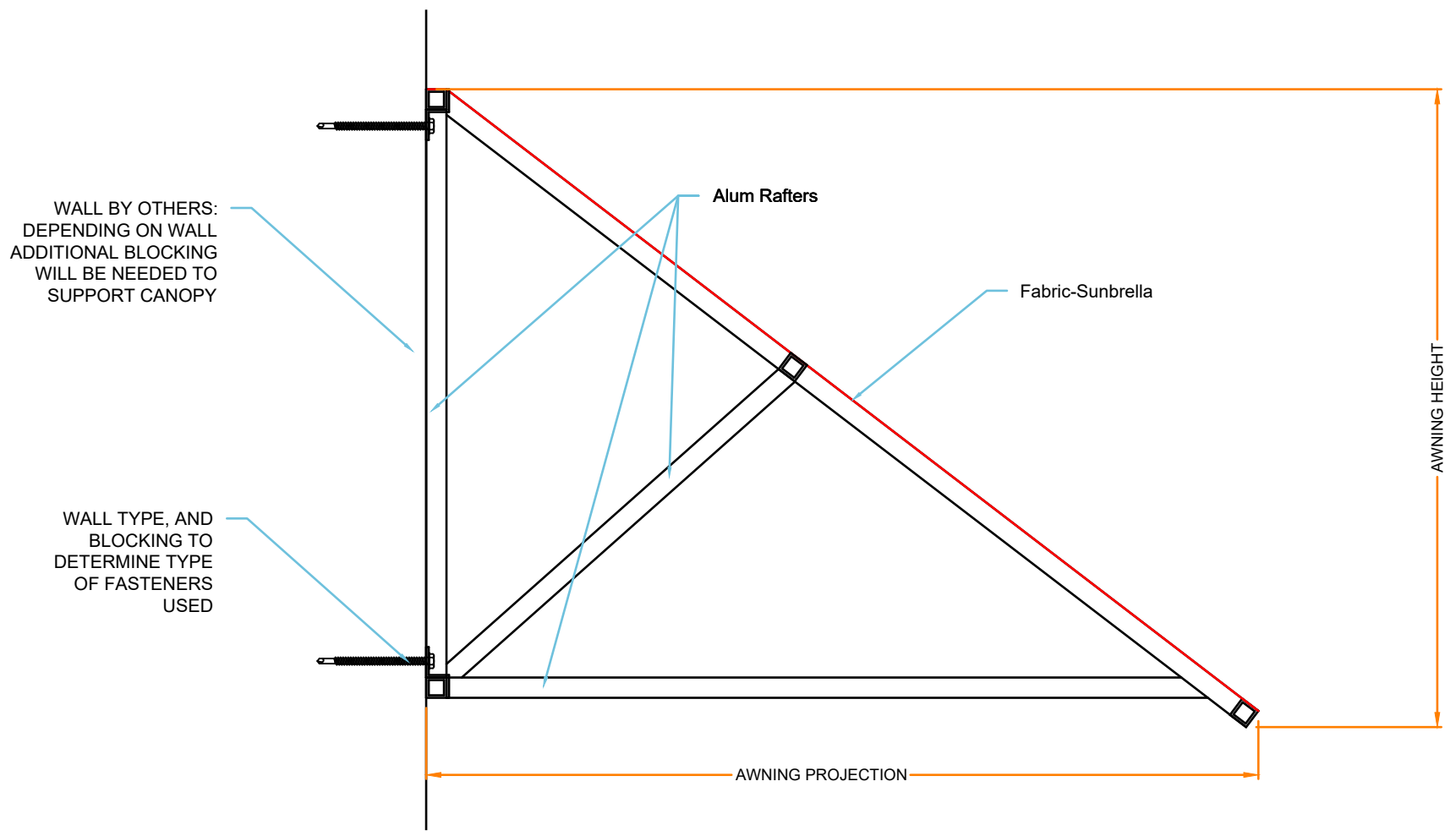
AWNING SECTION VIEW
