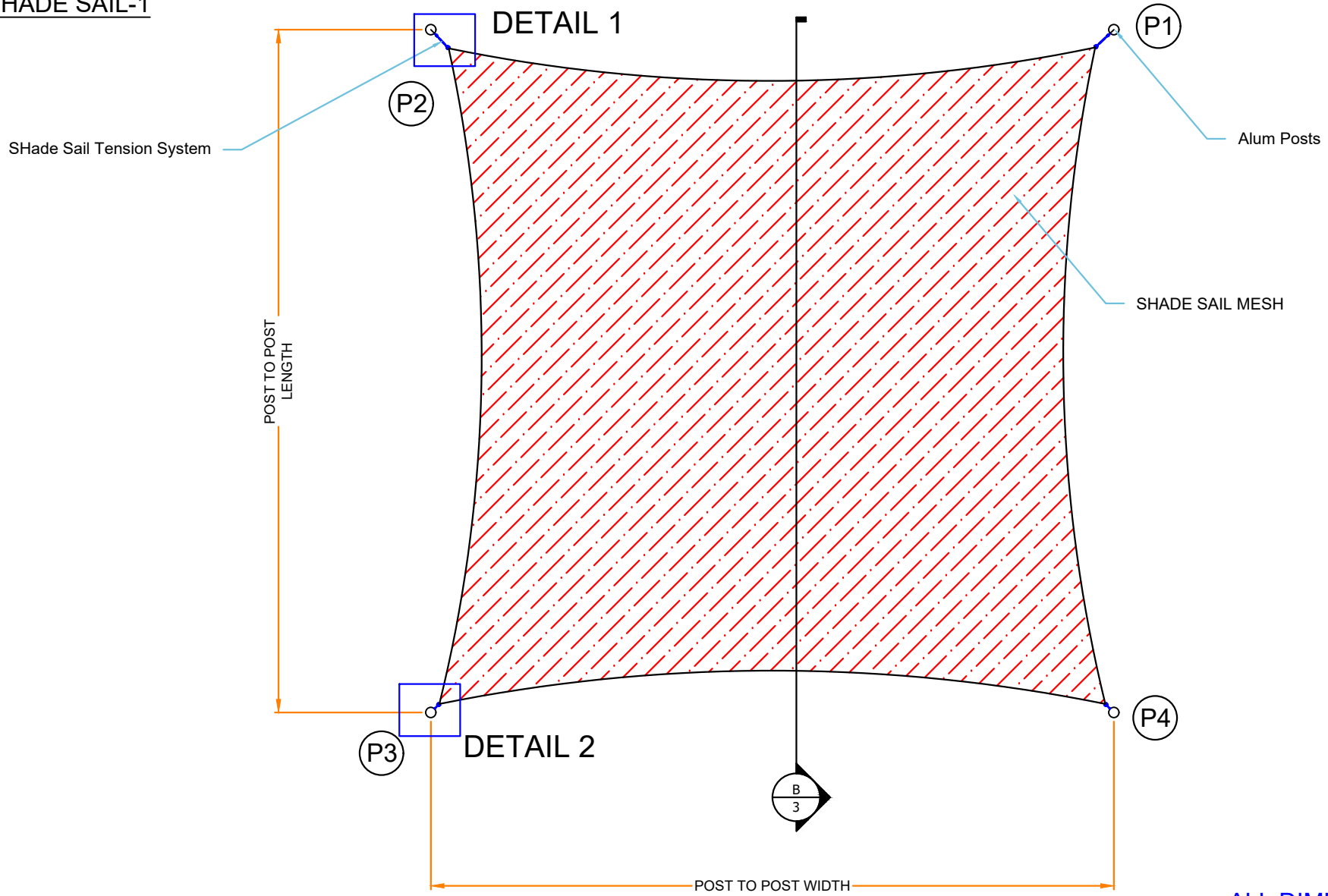
SHADE SAIL OVER VIEW
