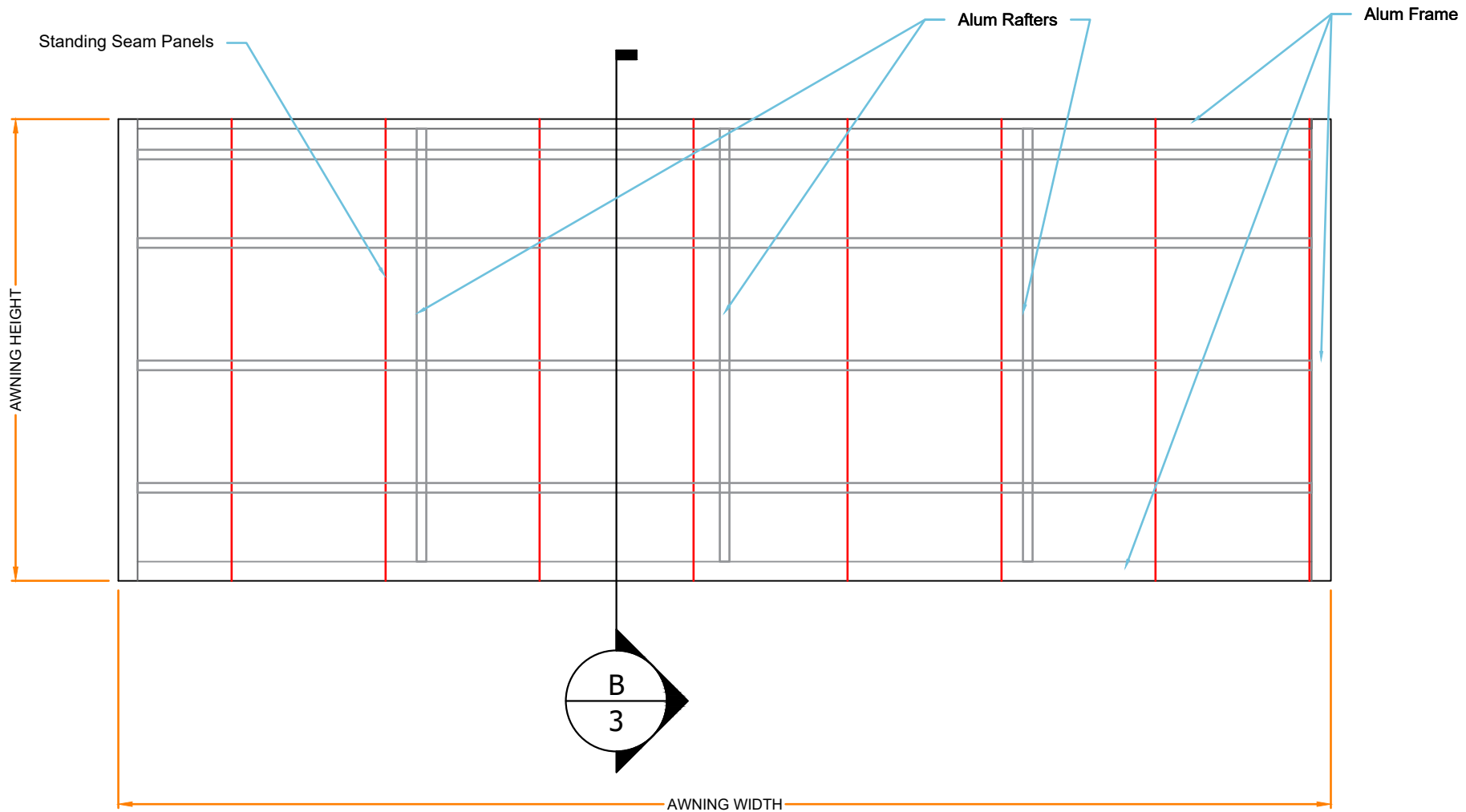
AWNING FRONT VIEW
