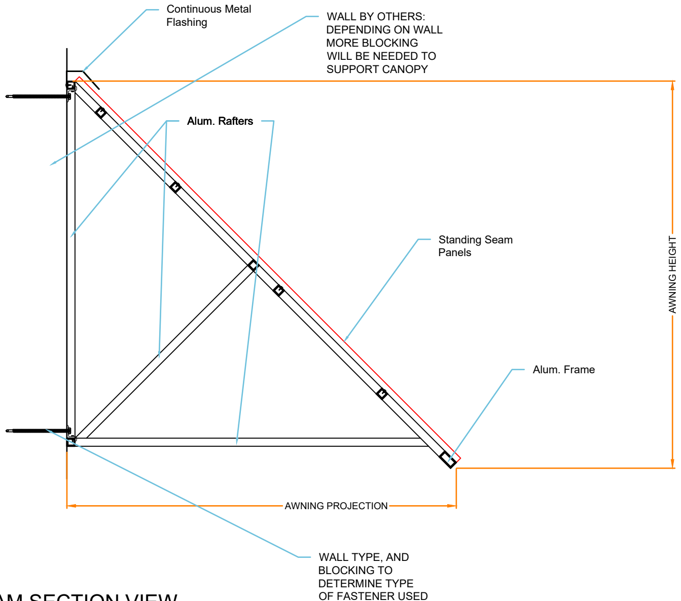
STANDING SEAM SECTION VIEW
